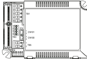
Terminal Pin No. Assignment(TB3)
